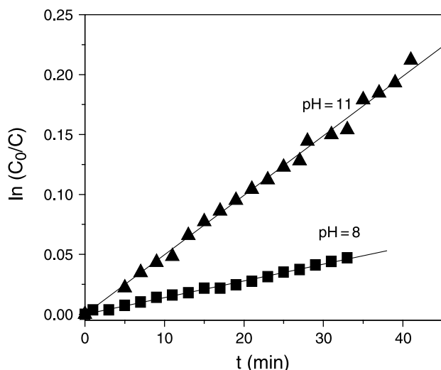
Fig. 3. Effect of the pH on the profiles of oxygen uptake by \alpha -Chymo upon PN-sensitized photoirradiation, in buffer at (■) pH = 8, (▲) pH = 11 [ \alpha -Chymo] = 1 \times 10^{-5} M
