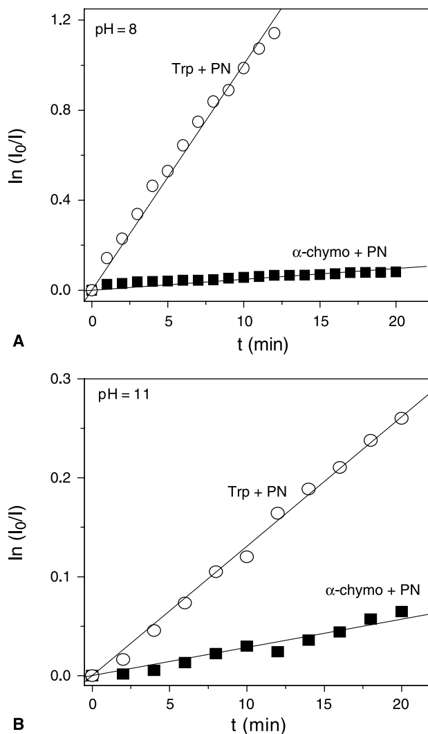
Fig. 2. First order plot consumption of \alpha -Chymo upon PN-sensitized photoirradiation for (○) Trp and (■) \alpha -Chymo in Buffer: (A) pH = 8 and (B) pH = 11. \lambda_{\text{em}} = 330 nm and 334 nm, respectively. I_0 and I represent the values of the respective maxima intensity in the fluorescence spectra at different irradiation times. \lambda_{\text{exc}} = 280 nm
