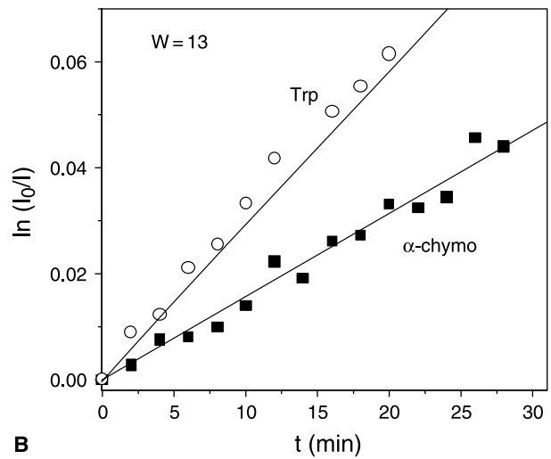
Fig. 6. First order plot consumption of \alpha -Chymo upon PN-sensitized photoirradiation for (O) Trp and (■) \alpha -Chymo in Reverse Micelles of water/AOT/n-heptane, at \text{pH}_{\text{ext}} : (A) 8 at W = 13 and 30 and (B) 11, W = 13 . I_0 and I represent the values of the respective maxima in the fluorescence spectra at different irradiation times. [\text{AOT}] = 0.1 \text{ M} , [\alpha\text{-Chymo}] = 2 \times 10^{-5} \text{ M}
